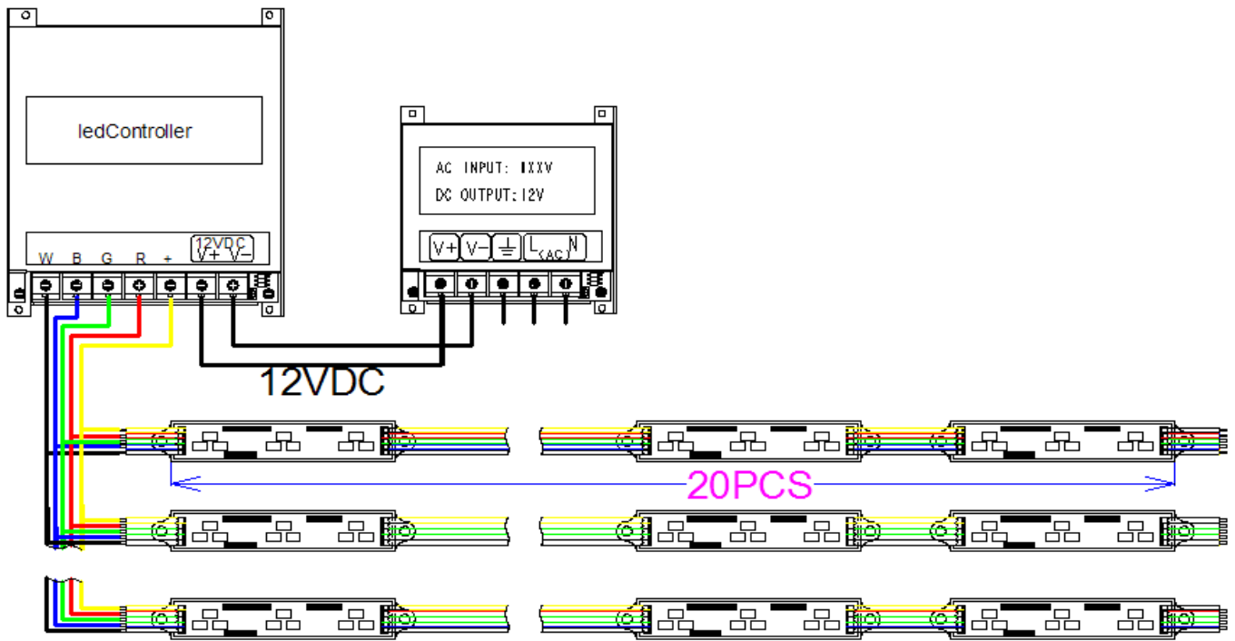
Wiring diagram
